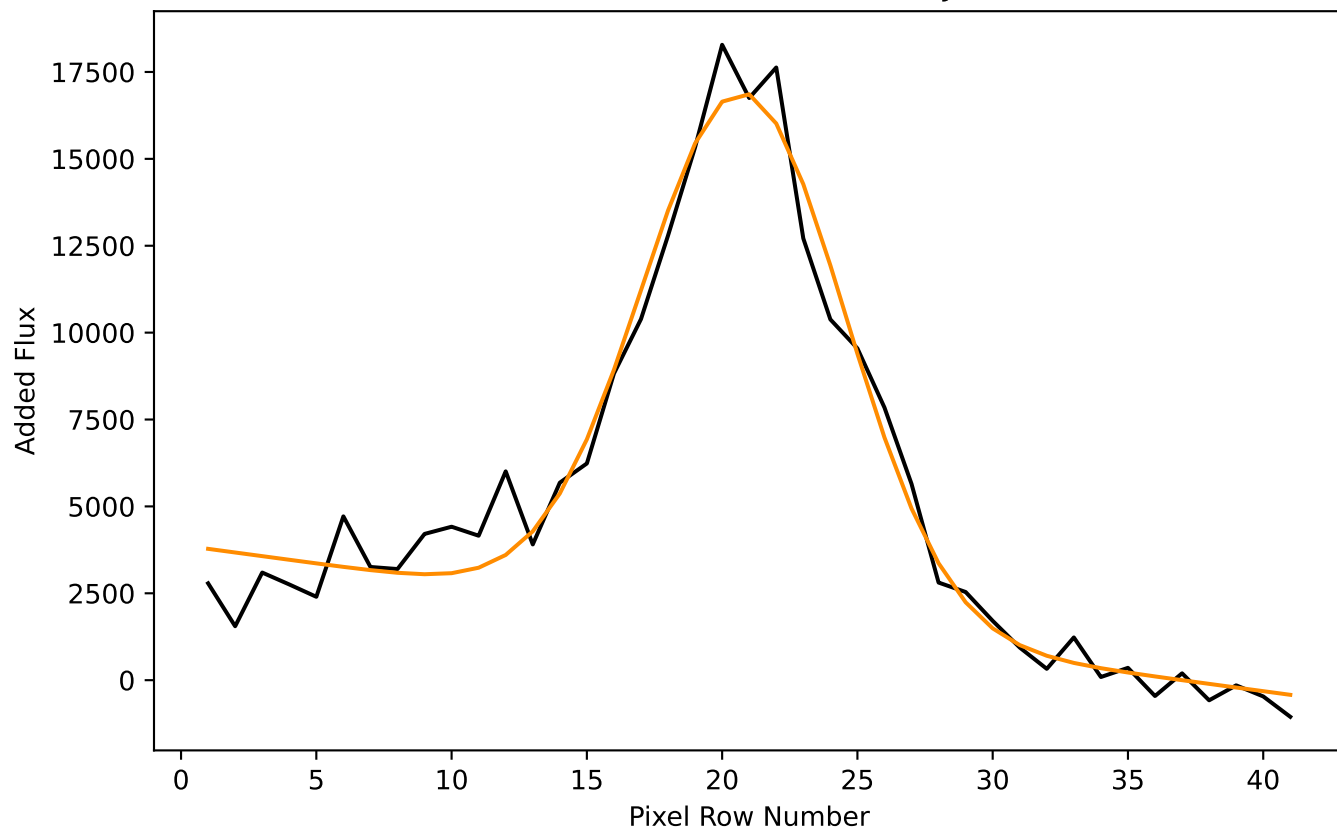
Column 870 Fit from Flux Calibrated J0800+3743
